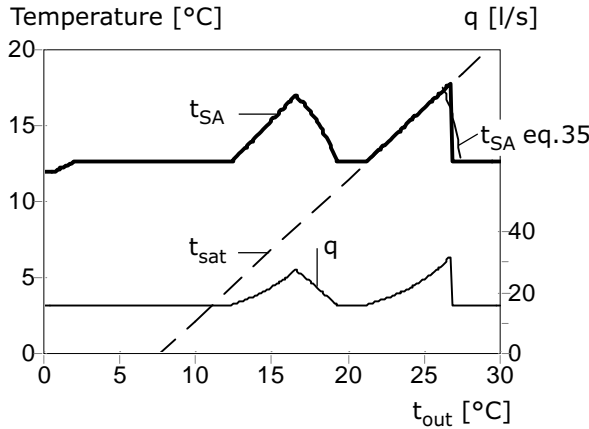
Fig. 10. Optimal supply air temperature ( t_{SA} ) and supply air flow, q , at different outdoor temperatures ( t_{out} ) and with a constant load, P_{load} = P_{internal} = 200 W ( U=0 ) corresponding to 15 W/m 2 floor area. \eta_t = 0.5 , q_{min} = 16 l/s. The dashed line is the saturation temperature ( t_{sat} ).
