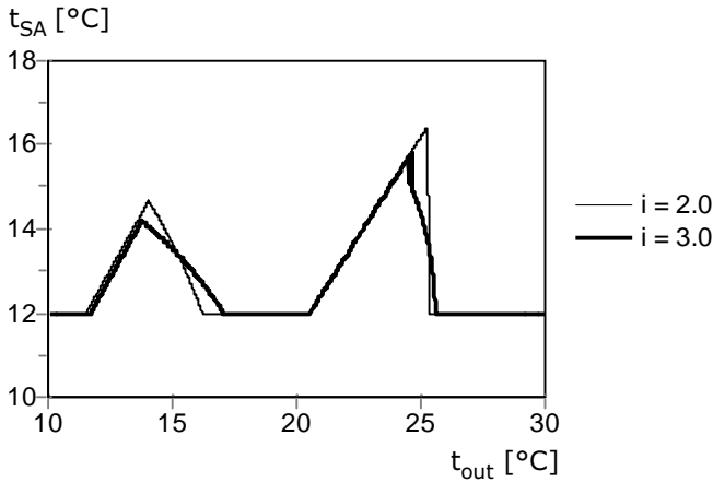
Fig. 16. Optimal supply air temperature with different exponents ( i ) in Eq. (5).
